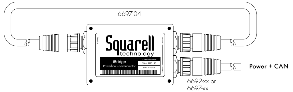
Fig. 2 Install when device power is used as powerline communications.
