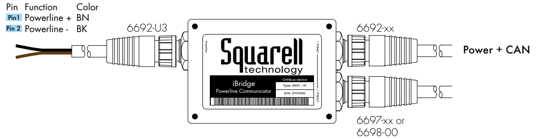
Fig.1 Install when device power is separate from powerline communications.
